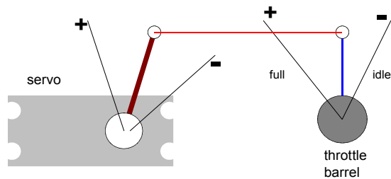
Diagram of suggested Servo arm offset.
