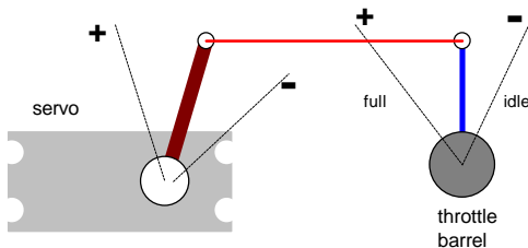
Diagram of suggested Servo arm offset.
